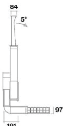
Side view, Slim motor on the back
