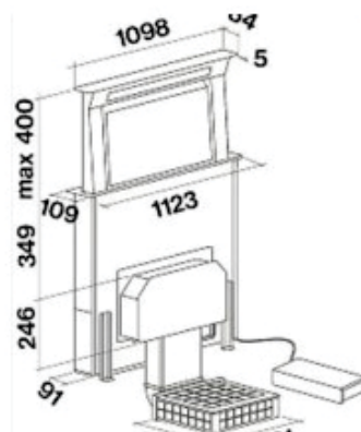
Filtering version (Slim motor) with Carbon.Zeo underbase filter (KACL.930)
