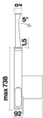
Side view, motor on the front
