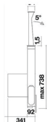
Side view, motor on the back
